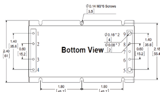
Full Brick Vicor Pinout/ 6-sided metal case
