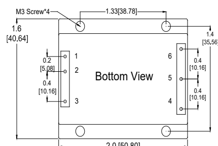
ESC Series Pinout
