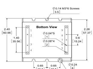
1/2 Brick DOSA Pinout/ 6-sided metal case
