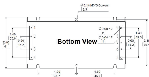
Full Brick Vicor Pinout/ 6-sided metal case
