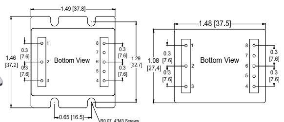
STB Series 6 sides aluminum case with flange DOSA Pinout
