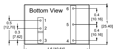
ESB Series Pinout
