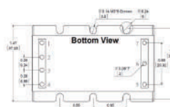
1/4 Brick VICOR Pinout/ 6-sided metal case
