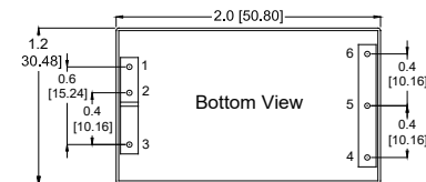
ESC Series Pinout
