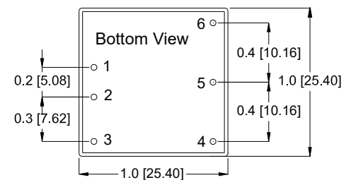
ESBS Series Flat
