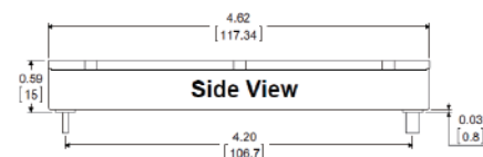
Full Brick Vicor Pinout
