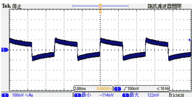
Figure 7 : Transient Response at Output step load ( V_{in} : Typical, 50\sim 75\% of output current; \Delta I_o/\Delta t = 1\text{A}/\mu\text{s} )
