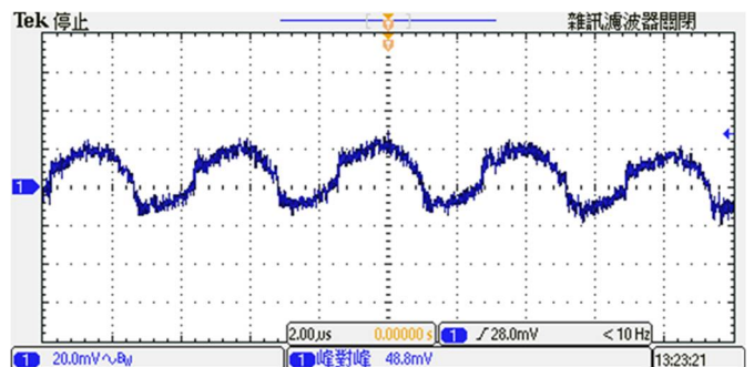
Figure 8 : Output Voltage Ripple & Noise at full load. ( V_{in} : Typical, With Output Capacitor to add 1\mu\text{F} MLCC)
