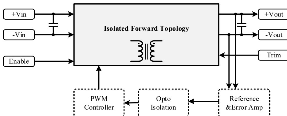
SQBF Series Block Diagram
