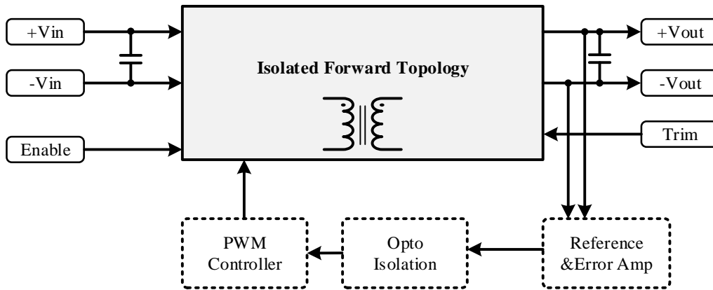
SQBS Series Block Diagram
