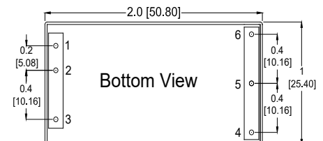
ESCS Series Pinout
