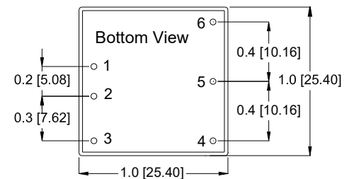
ESBS Series Pinout
