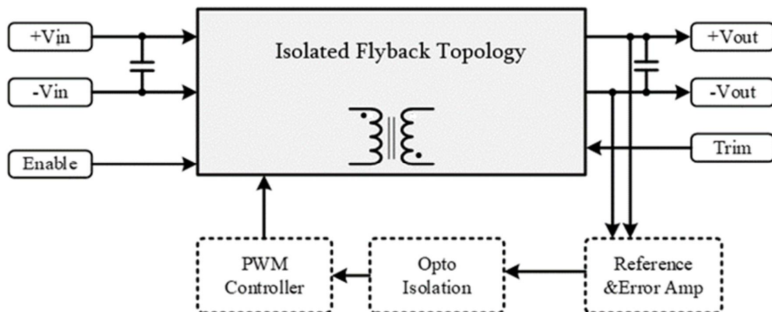
SFBS Series Block Diagram
