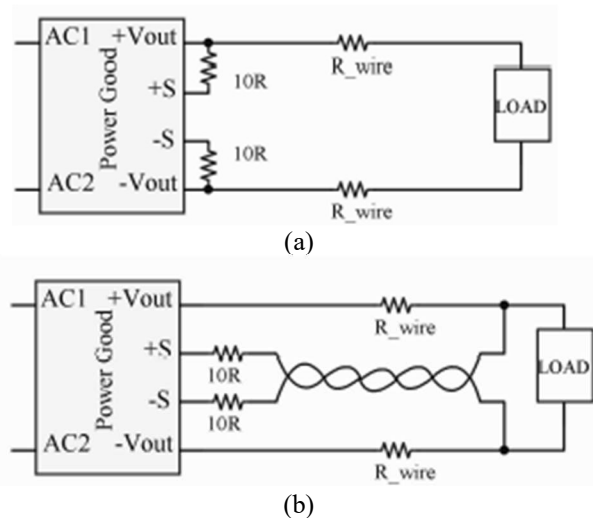
Figure 5. Remote Sense Circuit Configuration
