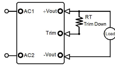
Figure 4. Trim down
