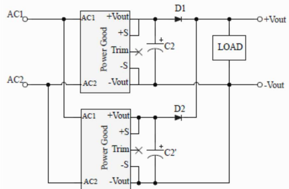
Figure 10. Redundant Connect
