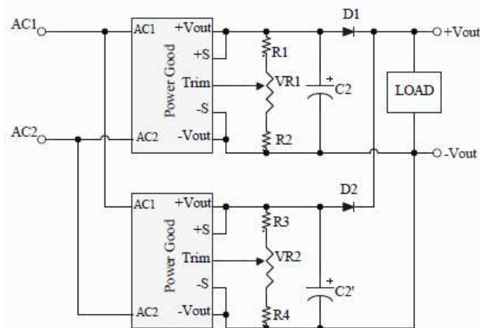
Figure 8. Connection in Parallel
