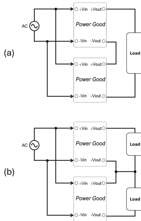
Figure 9. Redundant Connect
