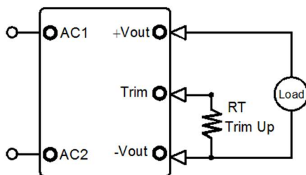
Figure 3. Trim up
