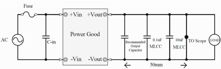
Figure 1. Measuring Output Ripple/Noise (20MHz bandwidth)
